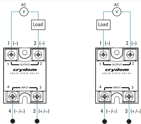
Generic AC Output SSRs Wiring Diagram
